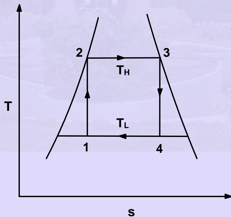
Fig.5.1 (b) T-s diagram
