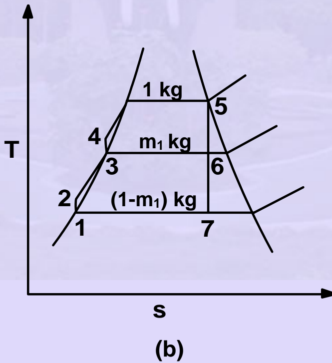
Fig.5.7. Open feed water heater cycle
