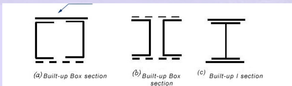
Fig 5.22: Cross Section Shapes for Built - up or fabricated Compression Members
