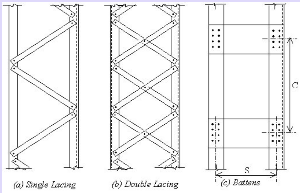
Fig. 5.23 Built-up column members
